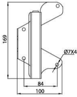
M02010255 Ürün No/Prod. No: 88 KOL BAĞLANTI MEKANİZMASI (M8 SOMUNLU) ARM CONNECTION MECHANISM (WITH M8 NUT)
